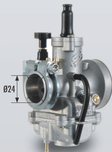
CP POLINI WITH KNOB CHOKE CLAMP CONNECTION POLINI CP STARTER ARIA A POMELLO, ATTACCO A FASCETTA
